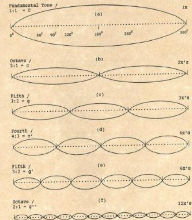
Figure 6.1 Musical intervals and corresponding frequency ratios.
